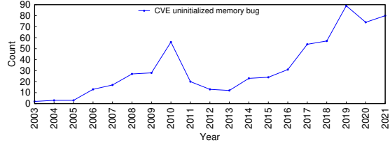
Figure 5: CVE uninitialized memory bugs reported over years
